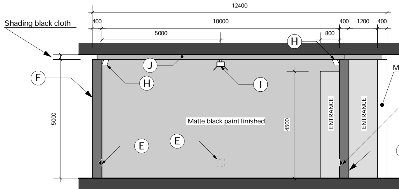
PROJECTION ROOM A-A' Section
